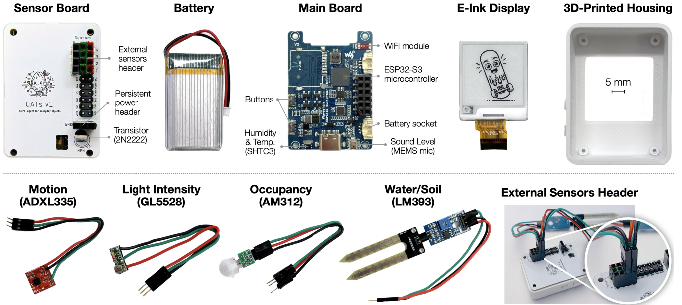
Figure 4: Top: The major hardware components of an OAT. Bottom: OATs are extensible with external sensors. We created a proof-of-concept suite of sensors that plug into a color-coded header on the back of an OAT device.
