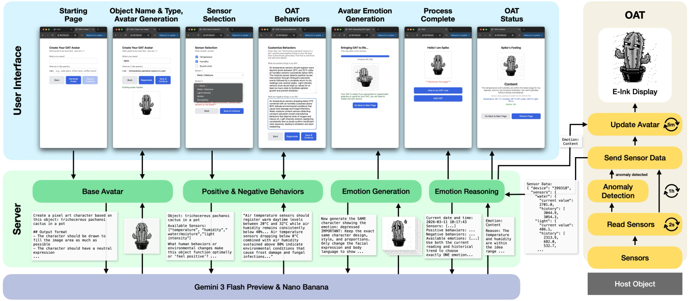
Figure 2: Block diagram of major processes and information flows. A photo of this example OAT can be seen in Figure 1.
