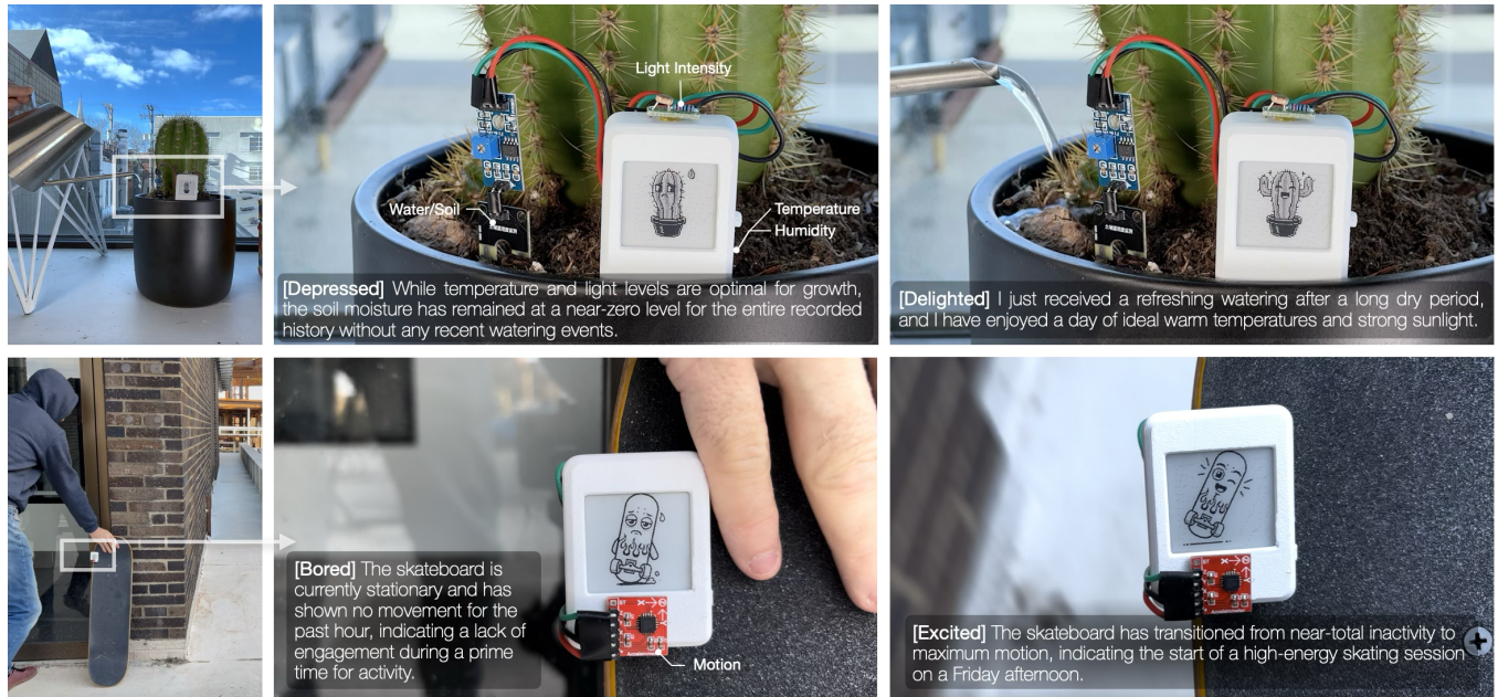
Figure 1: We created a toolkit that allows users to easily create Tamagotchi-like, expressive proxies for inanimate everyday objects, which we call Object-Agent Twins (OATs). Top: an OAT for a cactus, initially depressed due to a lack of water, becomes delighted when watered. Bottom: A bored skateboard becomes excited when the user begins to ride it. See also Video Figure.
