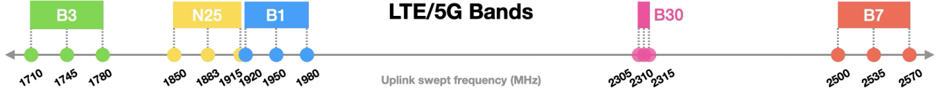
Figure 3: For each antenna, we measure performance at 3 frequencies across 5 different LTE and 5G cellular bands (B1, B3, B7, B30, N25), spanning from 1.7 to 2.6 GHz.
