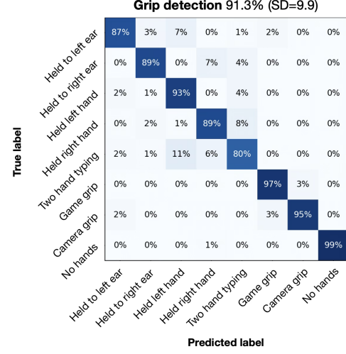
Figure 16: Grip pose detection confusion matrix.
