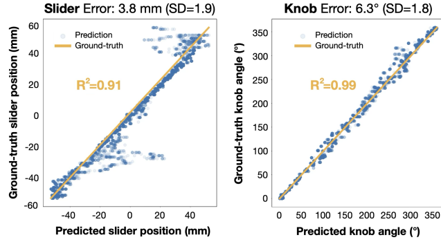
Figure 18: Scatter plots of predicted vs. ground truth values for slider position and turn knob angle. See also Figure 13.
