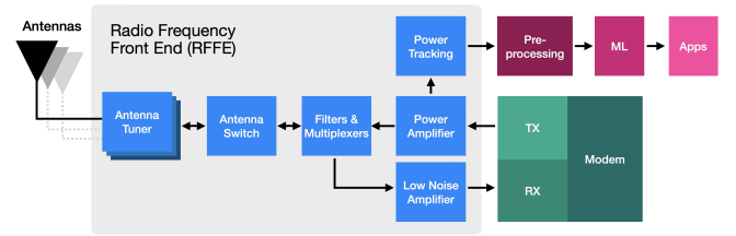
Figure 2: Block diagram showing the major components of a typical cellular modem (adapted from [46]). Our software interfaces with the power tracking features of the RFFE, passing data to machine learning to power interactive features.
