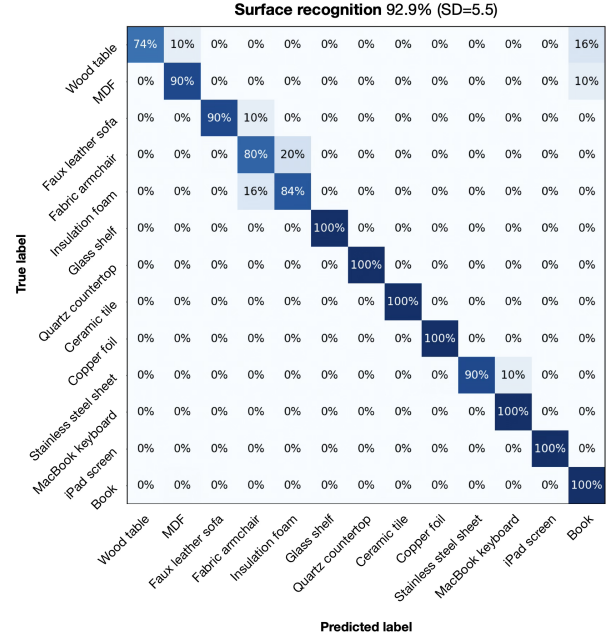
Figure 19: Surface recognition confusion matrix.
