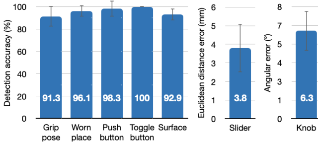
Figure 15: Accuracy summary for our five classification and two regression study results.
