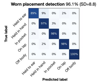
Figure 17: Worn-placement detection Confusion matrix.
