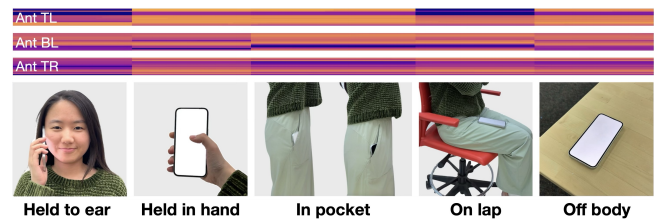
Figure 12: Bottom: Example worn placements detectable with smartphone RF sensing, including two in-pocket subclasses: screen facing inward and outward. Top: magnitude spectrograms (1.7–2.6 GHz, 3 antennas) recorded as a user performed each placement in sequence.
