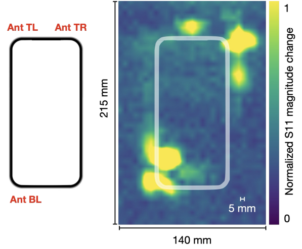
Figure 5: Heatmap of S11 change in response to a proximate antenna (see setup in Figure 4). It is apparent that the sensing range is limited to the immediate volume around the device, ideal for applications such as grip pose and surface recognition. Longer-range use cases appear infeasible at present.
