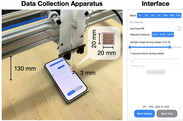
Figure 4: Left: CNC apparatus for probing the smartphone’s RF field. We use a wide-band monopole antenna, measuring 20 \times 20 mm, which was incrementally translated 3 mm above the phone screen, across a 140 \times 215 mm area. Cellular antenna performance was measured at each position, producing a spatial visualization of antenna performance (Figure 5). Right: Screenshot of our RFFE control interface.
